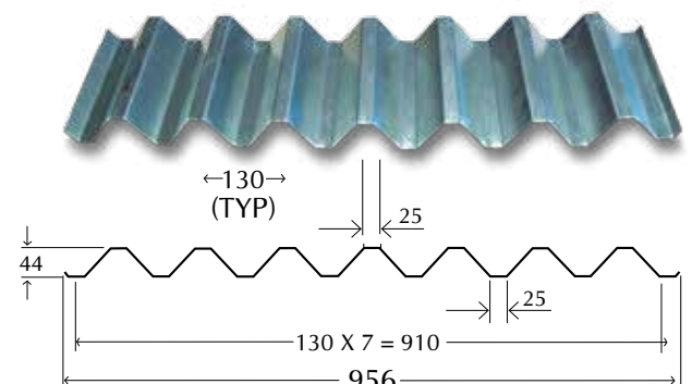
EZYDEK™ 44 Profile *All dimensions mentioned are in mm
