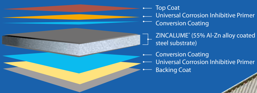
Cross Section of COLORBOND® steel
