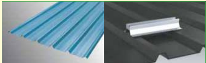
TRIMDEK® 1015 and Solar Mounting Clip
